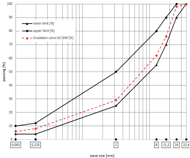
Fig. 2. Gradation curve of the AC 16W KR 3-4 mineral mixture
